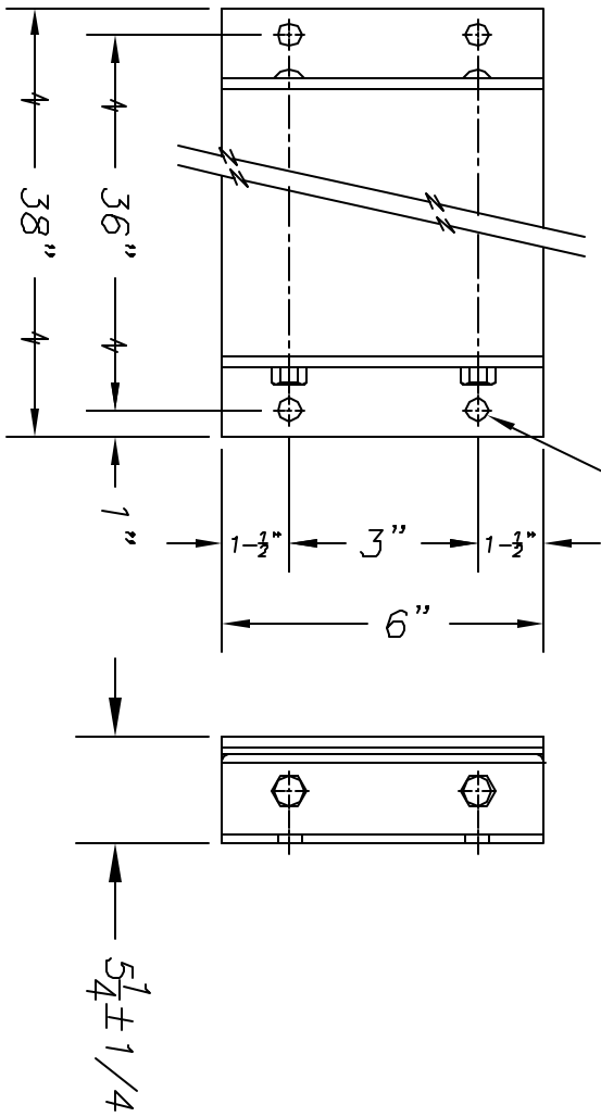
FRONT VIEW
