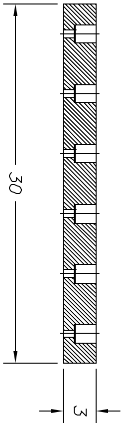
TOP VIEW
